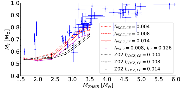
Figure 12. Initial-final mass relation for models where CBM is applied at both boundaries for several values, black lines are all calculated at Z=0.02 , all others at Z=0.008 . Data points are from the semi-empirical IFMR of Cummings et al. (2018) .
