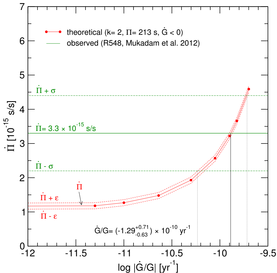
Figure 3. Same as figure 2 for R548. The effective temperature of the models is T_{\text{eff}} \sim 11\,630 K.
