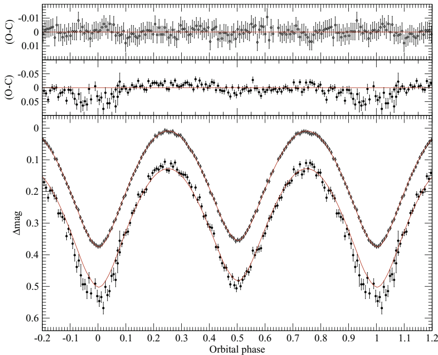
Fig. 3. Light curve fits assuming an overcontact binary system made of two degenerate post-AGB cores. B- and I-band light curves are shown in the lower panel using filled and open circles, respectively. Red lines are the best-fit models for each band. Residuals are shown in the upper panels. Note the different scale for each band. (For interpretation of the references to color in this figure legend, the reader is referred to the web version of this article).
