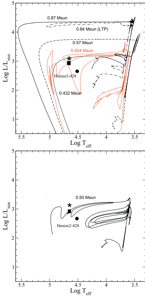
Fig. 1. Relevant evolutionary tracks (see text for details). Marked are the location of each of the two identical stars of Henize 2–428 according to the model of Santander-García et al. (2015), filled circle, and the central star in our proposed scenario when the distance is D = 1.4 kpc (filled square) and when D = 1.8 kpc (asterisk).
