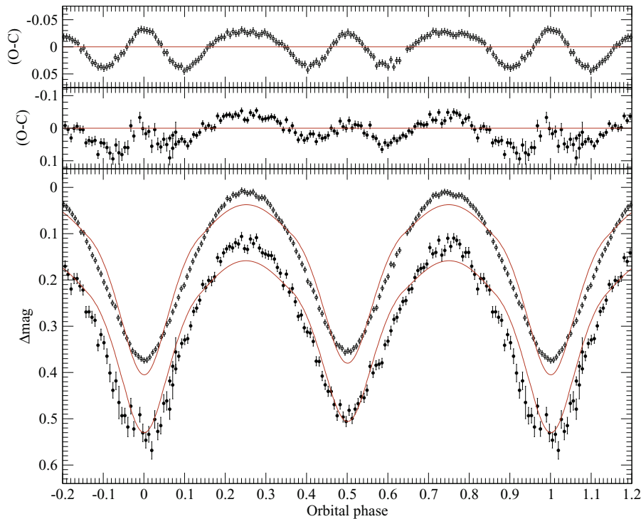
Fig. 2. Light curve fit assuming a semidetached binary system made of a degenerate core and a main sequence companion, with the primary component filling the Roche lobe. B- and I-band light curves are shown in the lower panel using filled and open circles, respectively. Red lines are the best-fit models for each band. Residuals are shown in the upper panels. Note the different scale for each band. (For interpretation of the references to color in this figure legend, the reader is referred to the web version of this article).
