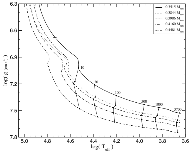
Figure 14. Same as Fig. 13 but for 0.3515, 0.3844, 0.3986, 0.4160 and 0.4481 M_{\odot} O-WD models. We plot isochrones (in Myr units) for 10, 30, 100, 500, 1000 and 3700.
